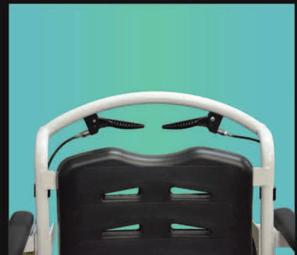
Quick release black clips can be removed and placed in adjacent holes to change caster height
